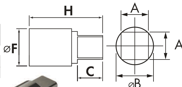
Custom Fabricated Stem Extensions
